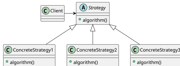
Figure 320: The UML diagram of the strategy pattern
